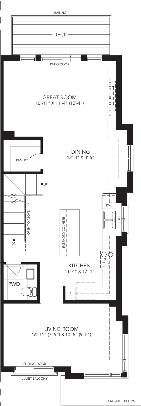
MAIN FLOOR PLAN A
