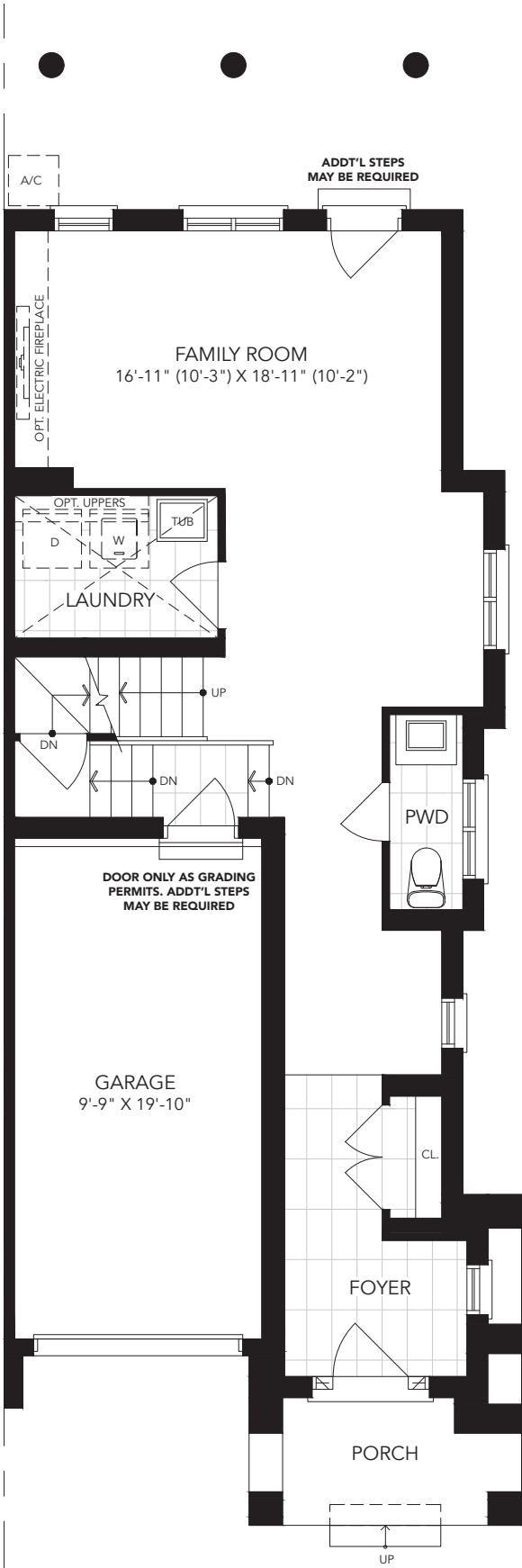
GROUND FLOOR PLAN A
