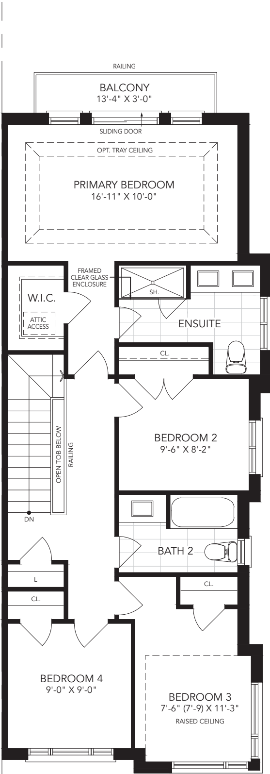
UPPER FLOOR PLAN A
