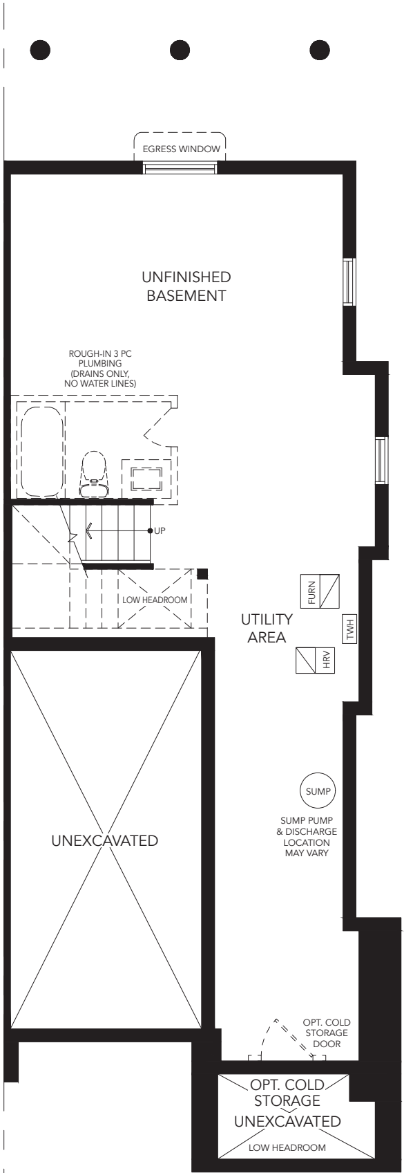
BASEMENT PLAN A
